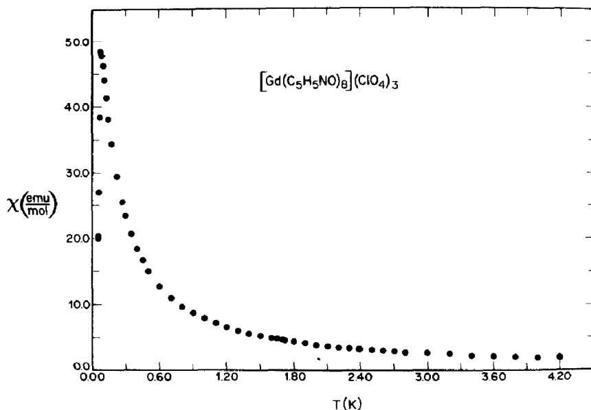
Fig. 5. Magnetic susceptibility of polycrystalline [\text{Gd}(\text{C}_5\text{H}_5\text{NO})_8](\text{ClO}_4)_3 . From ref. 49.
